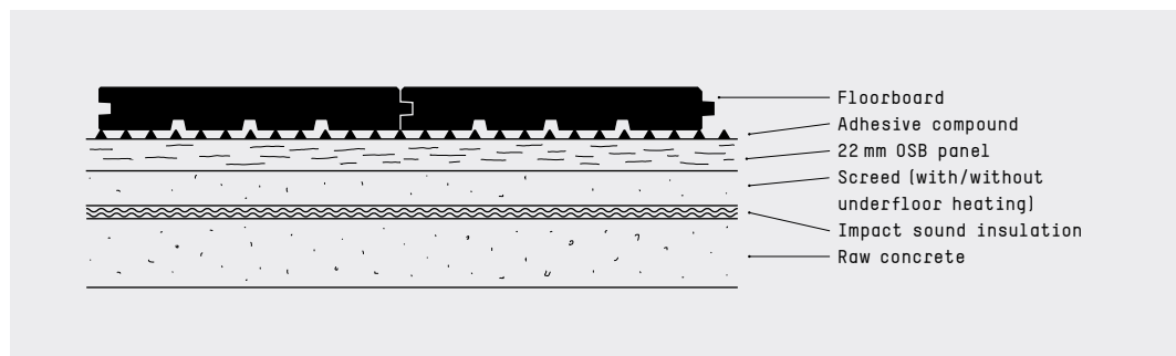
Figure 4: Gluing on OSB boards
