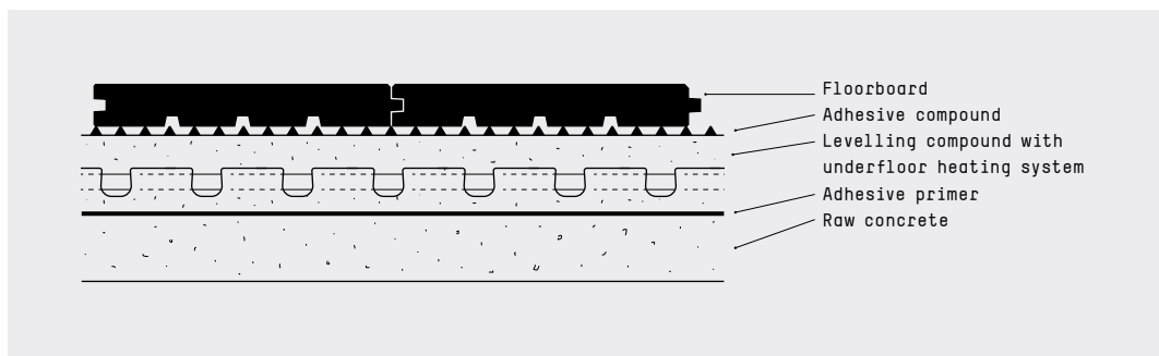
Figure 6: Screwing on thin-layer screed underfloor heating system
